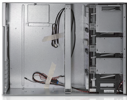
T-C25HD 2.5" hotswap hdd cages & slim ODD not included
